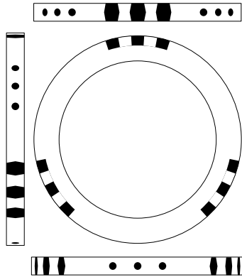
3 SMALL INSERT 5.54.011
