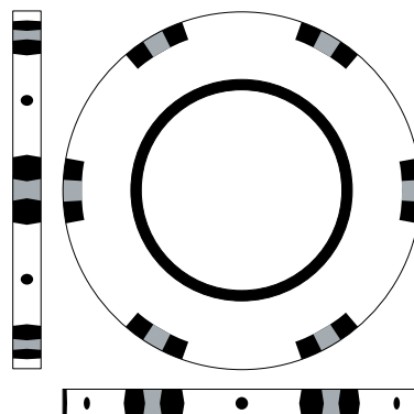
6 SMALL INSERT 5.34.013
