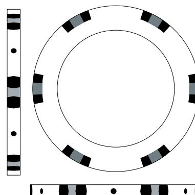
6 SMALL INSERT 5.84.013
